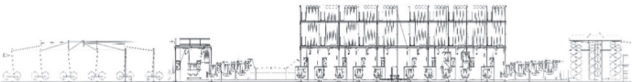
The sealed nitrogen reactors keep indigo in LEUCO-FORM (green). During its penetration, giving the possibility to be uniformed diffused into the fiber, reducing also the environmental impact.
